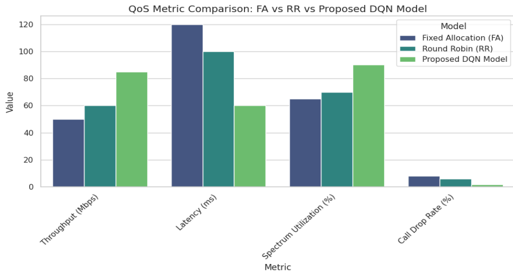
Figure 3: Performance Results of the Proposed Model
